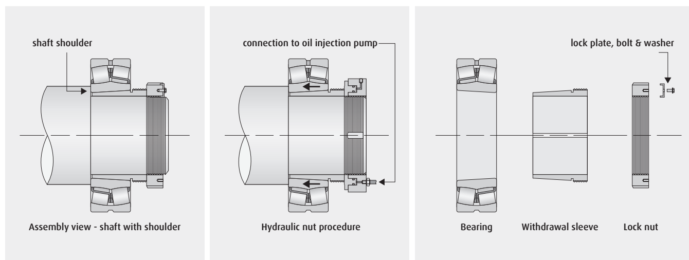
Fig. 19 - Spherical Roller Bearing Mounted with Withdrawal Sleeve on Cylindrical Shaft - Hydraulic Nut Method
